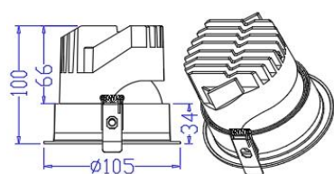
Trim type
